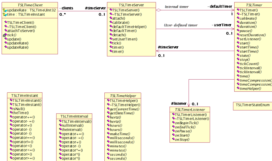
Figure 30 MapLink Time classes.
