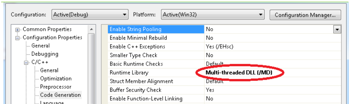
Figure 1 Release Runtime Library Setting
