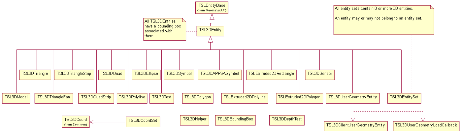
Figure 29 3D Entity Hierarchy
