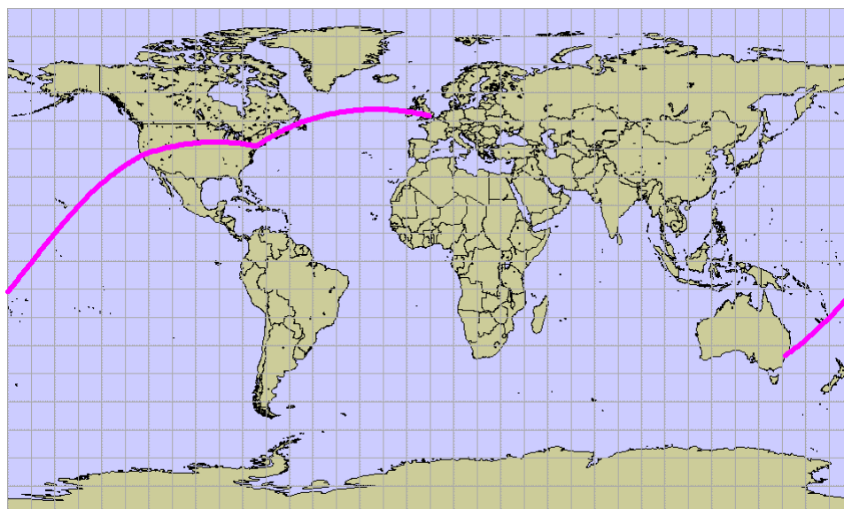
Figure 14 Single geodetic polyline with four points, travelling through Sydney, San Francisco, New York and London.
