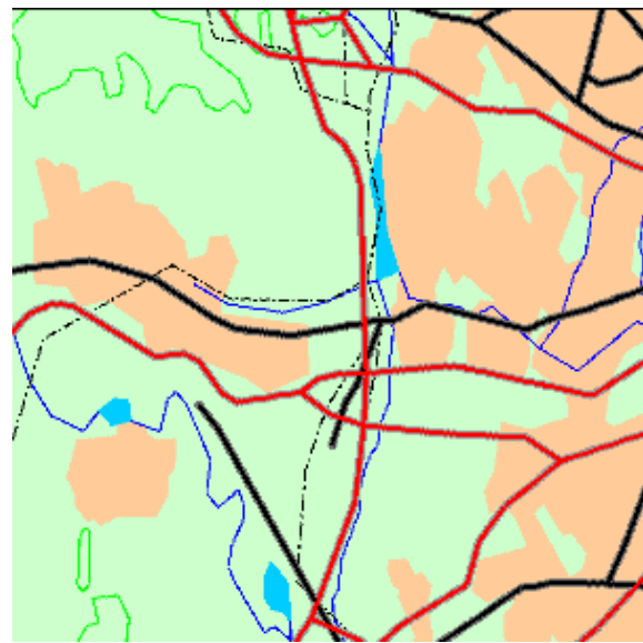
2x multisampling
