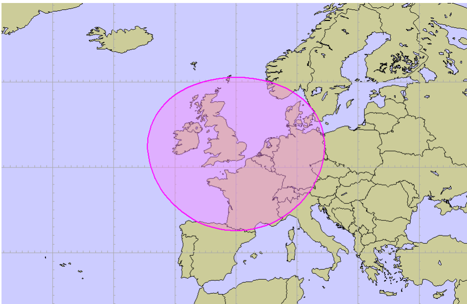
Figure 19 Geodetic ellipse centred on London; x- and y-radius 1000km
