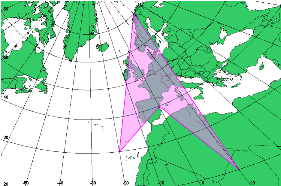
Figure 17 Four-point geodetic polygon, but on a gnomonic projection. In this projection, geodesics are straight lines, so the geodetic polygon looks like a standard polygon. The distortion in its shape is due to the centre of projection being off to one side of the geometry
