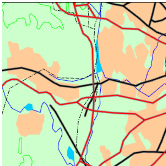
4x multisampling
