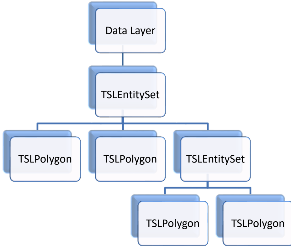
Figure 22 - Per Tile Storage Strategy
