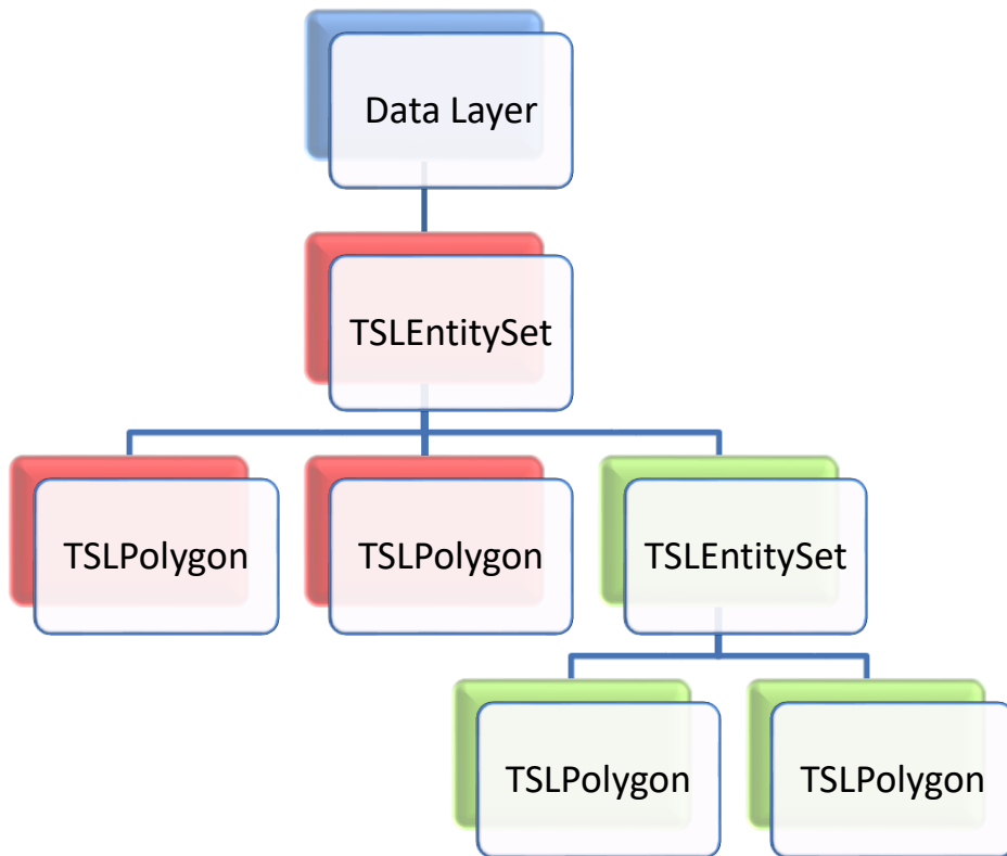
Figure 23 - Per Entity Set Storage Strategy
