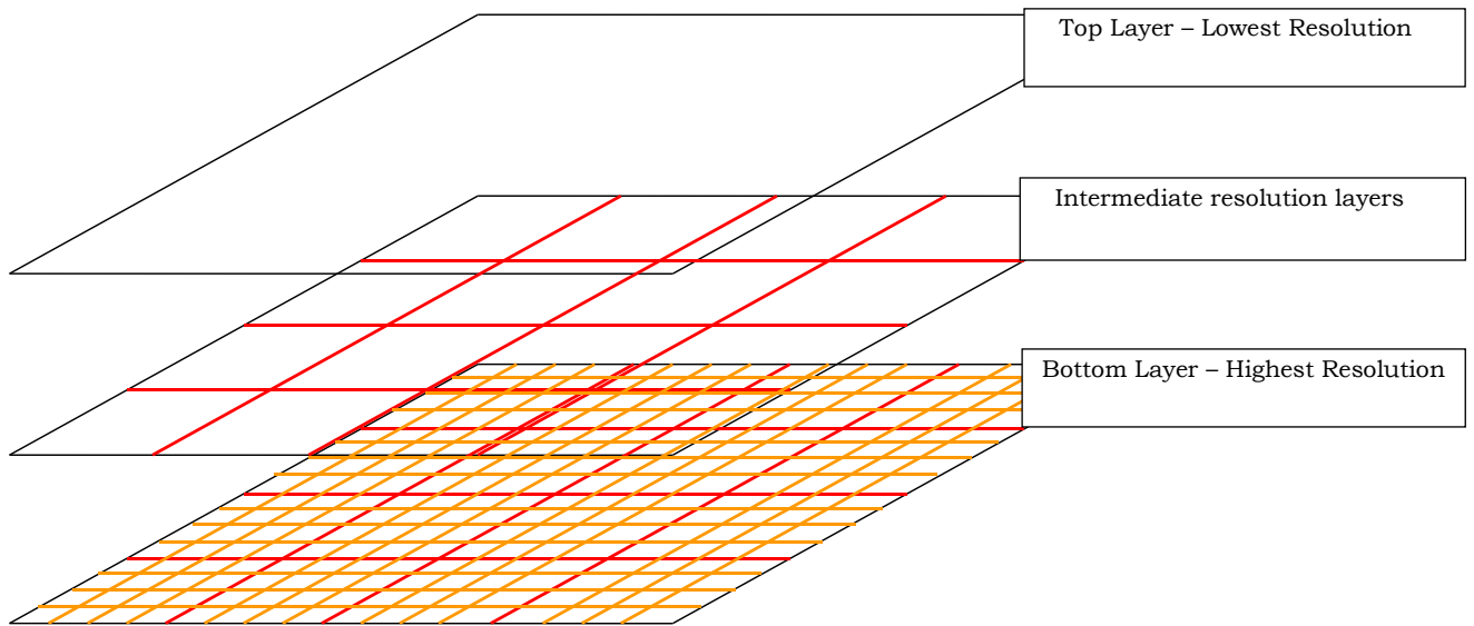
Figure 25 Terrain Pyramid
