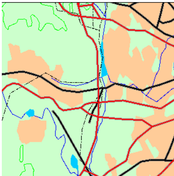
No multisampling
