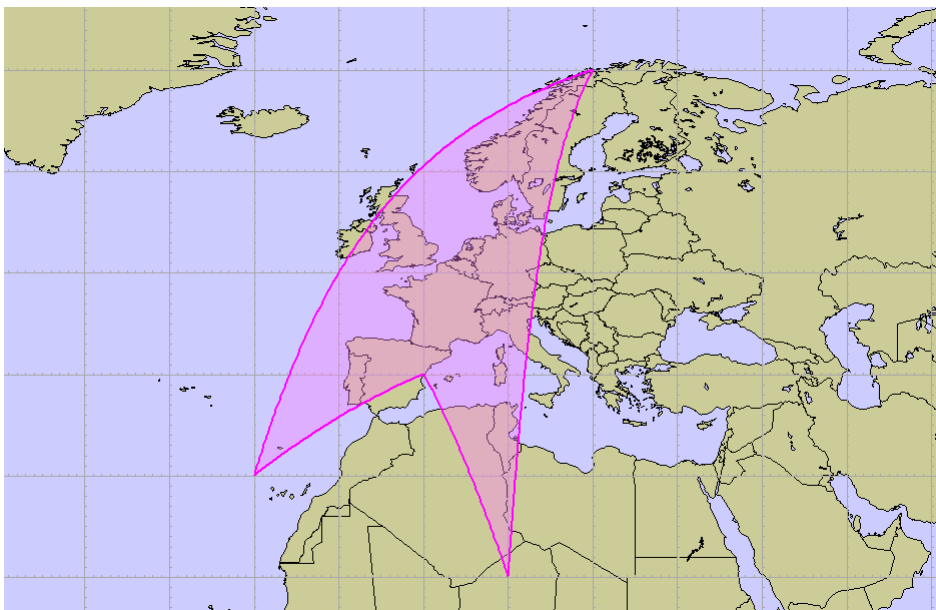
Figure 15 Four-point geodetic polygon
