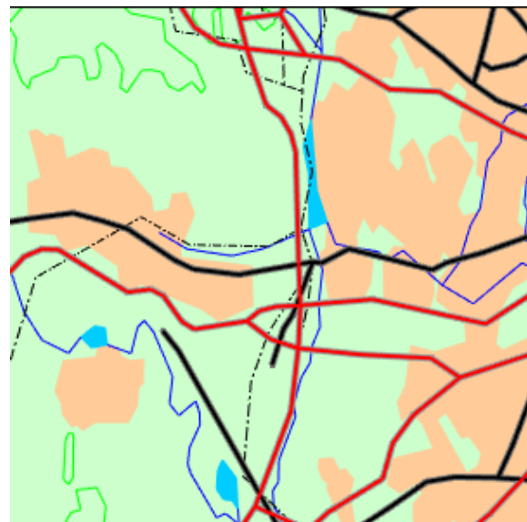
8x multisampling
