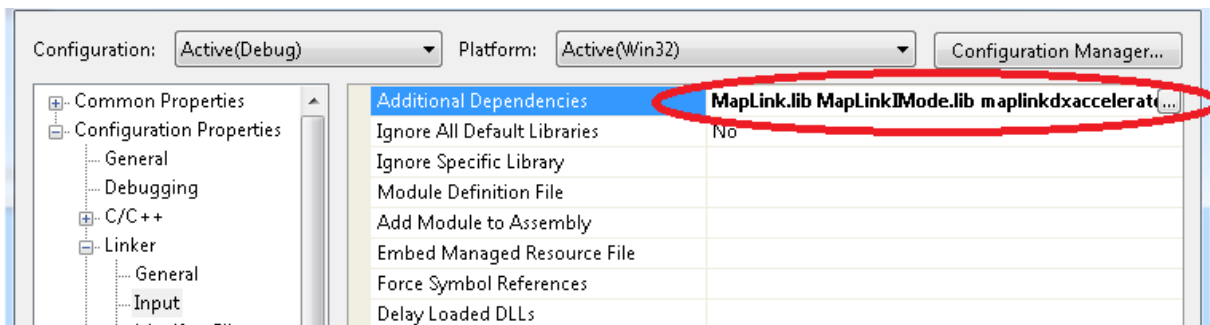
Figure 2 Additional Dependencies
