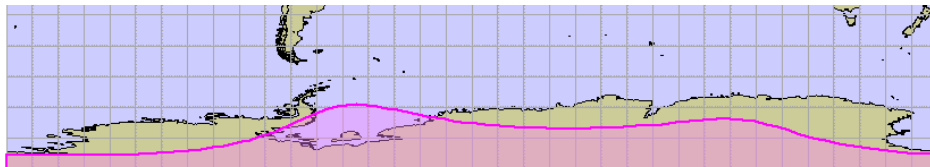
Figure 20 Geodetic ellipse centred on 85°S 0°E; x-radius 1000km, y-radius 2000km, rotation 60°.]
