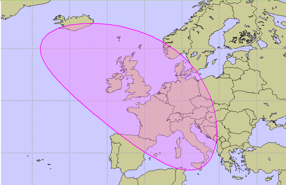
Figure 18 Geodetic ellipse centred on London; x-radius 1000km, y-radius 2000km, rotation 45°.
